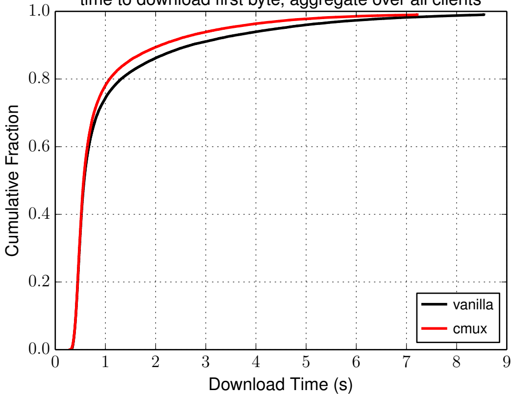
time to download first byte, aggregate over all clients
