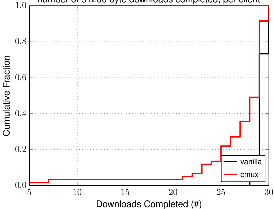
number of 51200 byte downloads completed, per client
