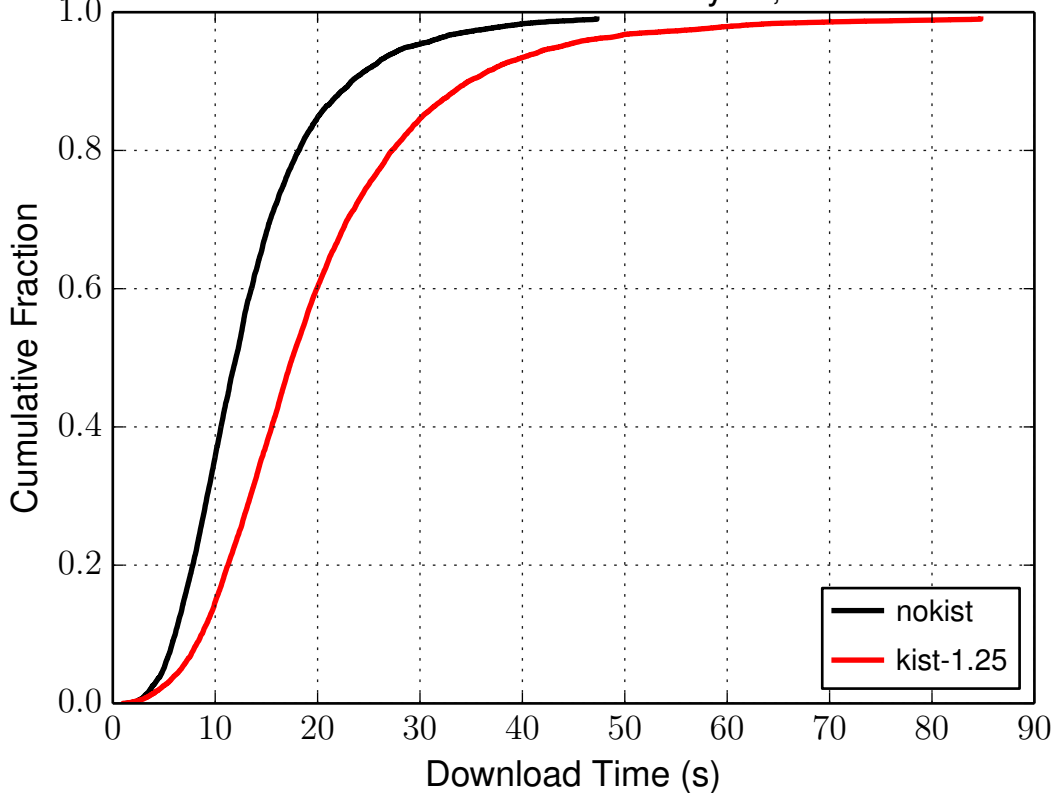
mean time to download 327680 bytes, each client
