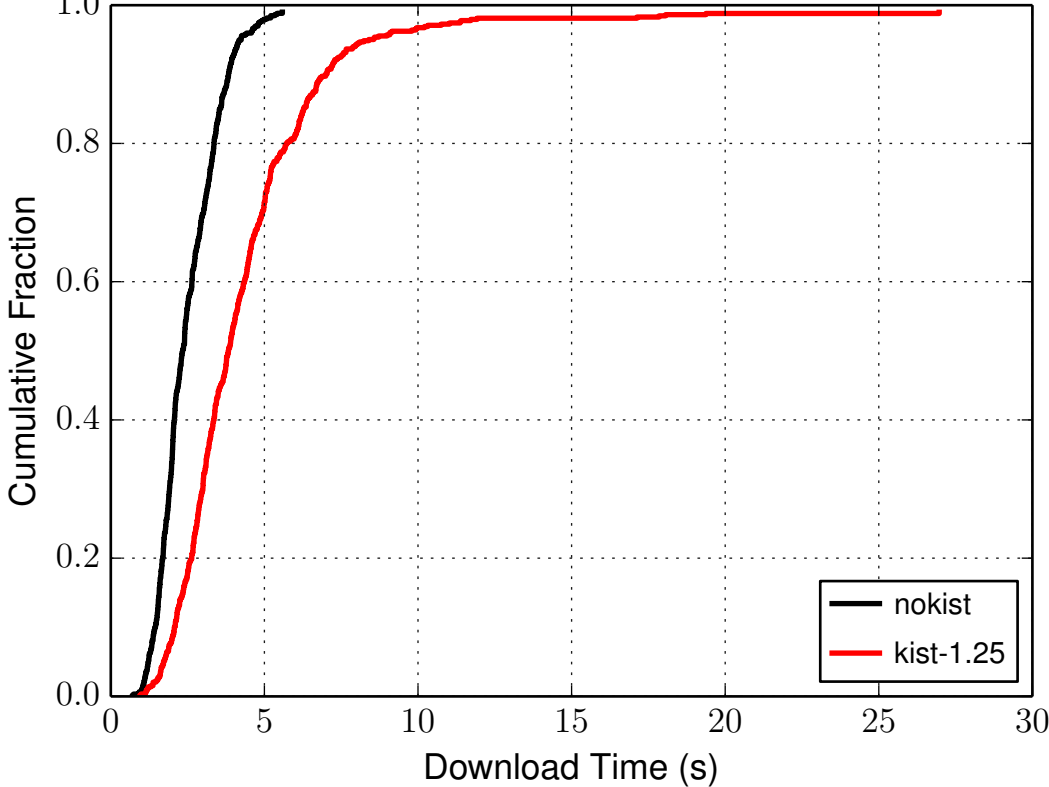
median time to download 51200 bytes, each client
