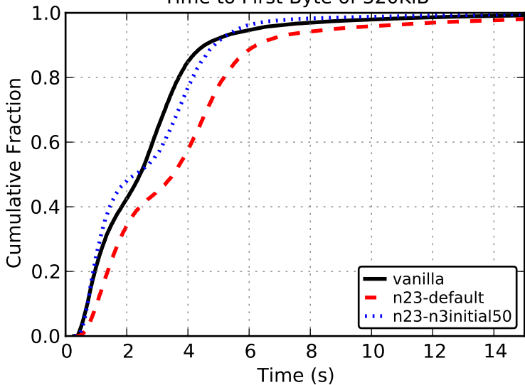
Time to First Byte of 320KiB
