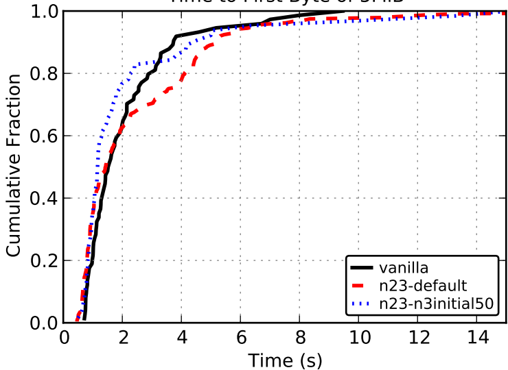
Time to First Byte of 5MiB
