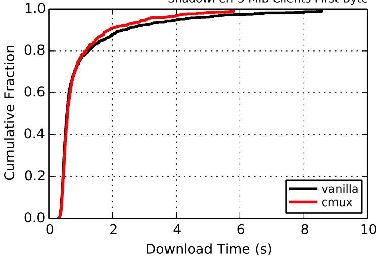
ShadowPerf 5 MiB Clients First Byte
