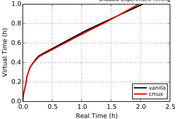
Shadow Experiment Timing
