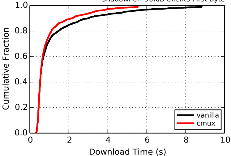
ShadowPerf 50KiB Clients First Byte
