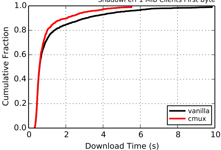
ShadowPerf 1 MiB Clients First Byte
