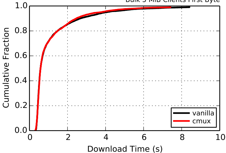
Bulk 5 MiB Clients First Byte
