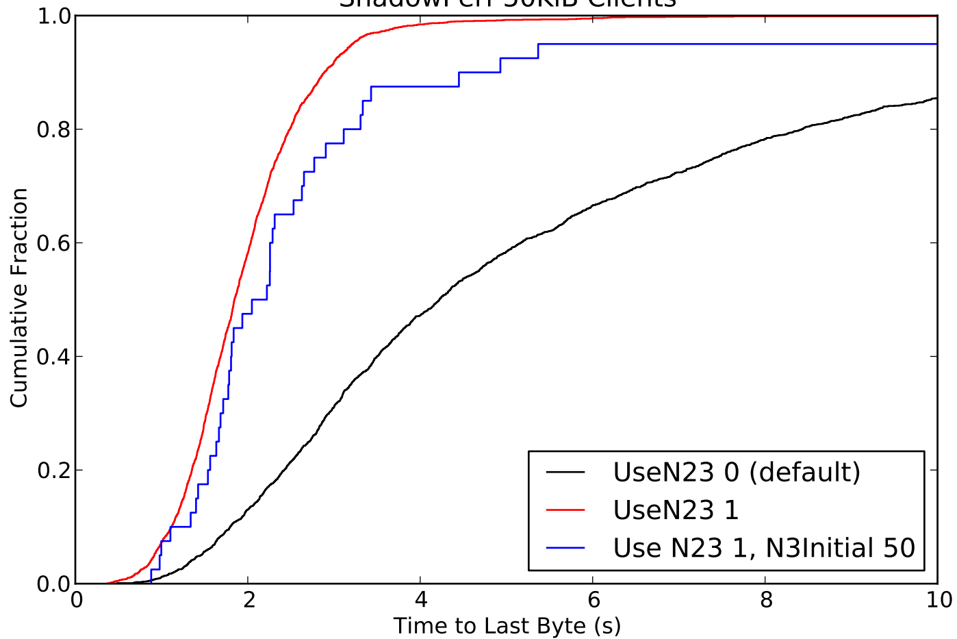
Simulation of N23 (arma/n23-4, commit fb5fdbf) ShadowPerf 50KiB Clients
