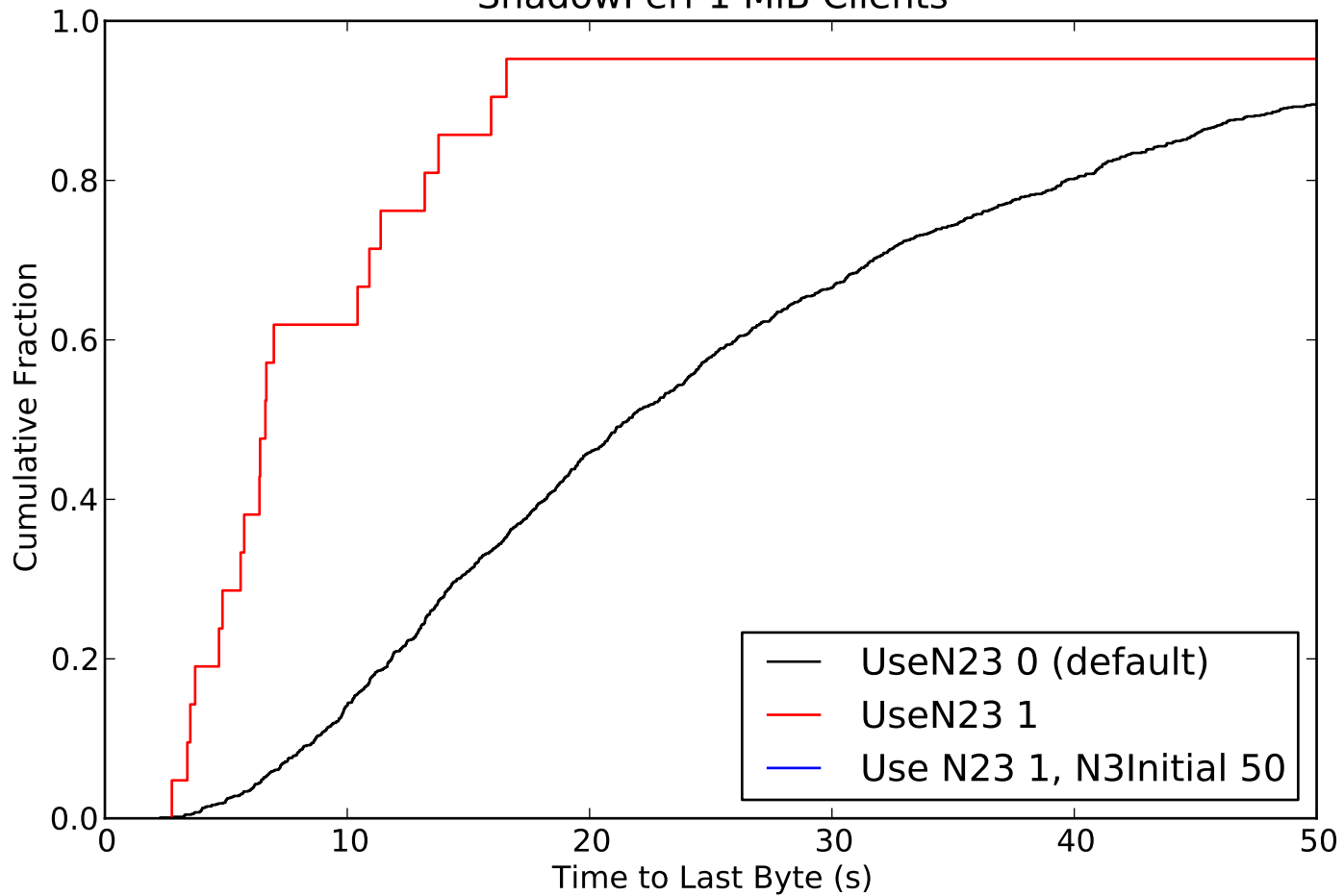
Simulation of N23 (arma/n23-4, commit fb5fdbf) ShadowPerf 1 MiB Clients
