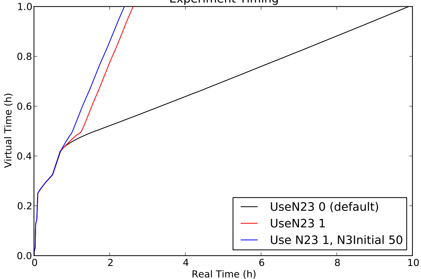
Simulation of N23 (arma/n23-4, commit fb5fdbf) Experiment Timing
