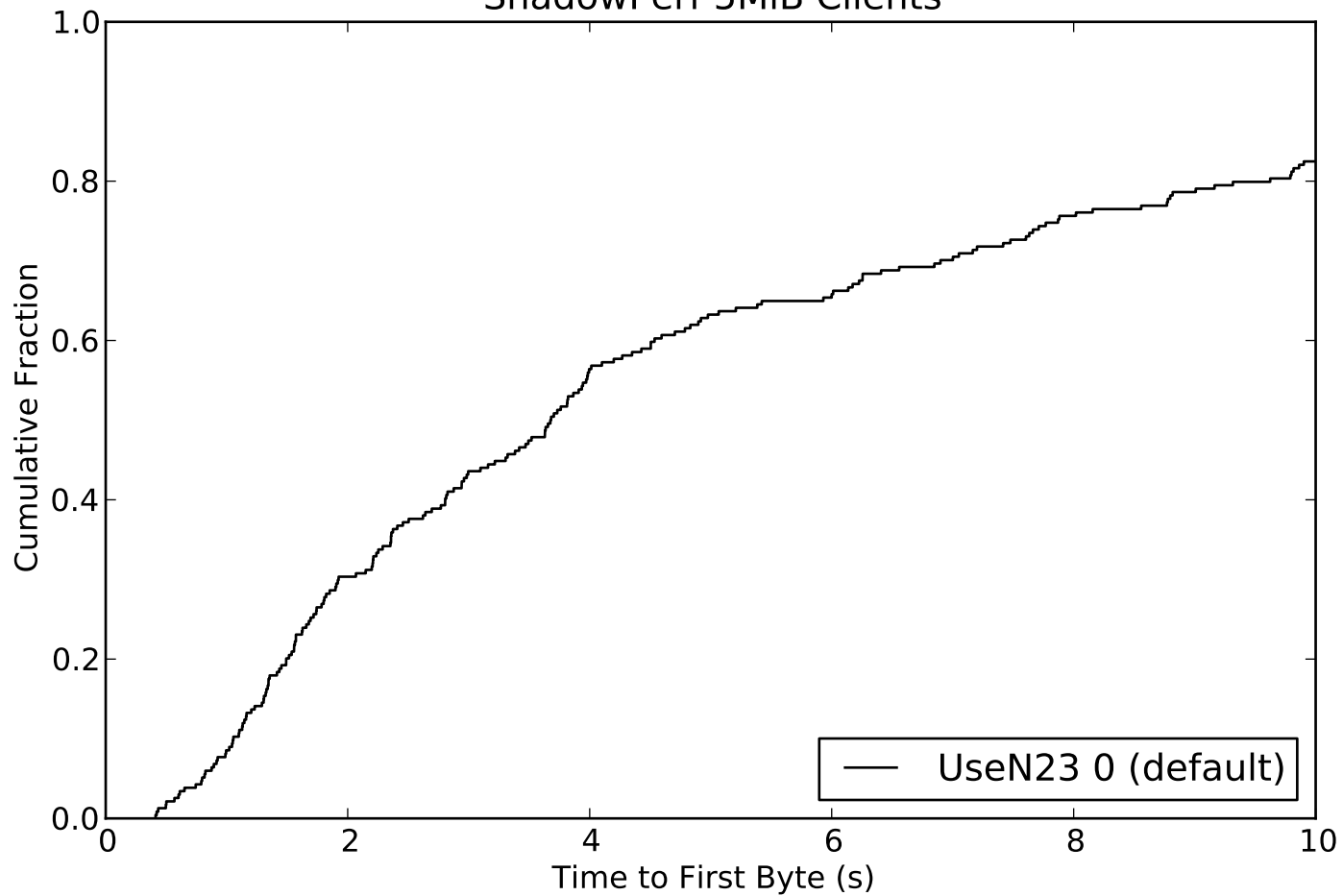
Simulation of N23 (arma/n23-4, commit fb5fdbf) ShadowPerf 5MiB Clients
