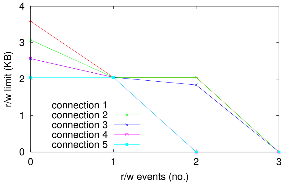
rate limit of 30KB (current algorithm)
